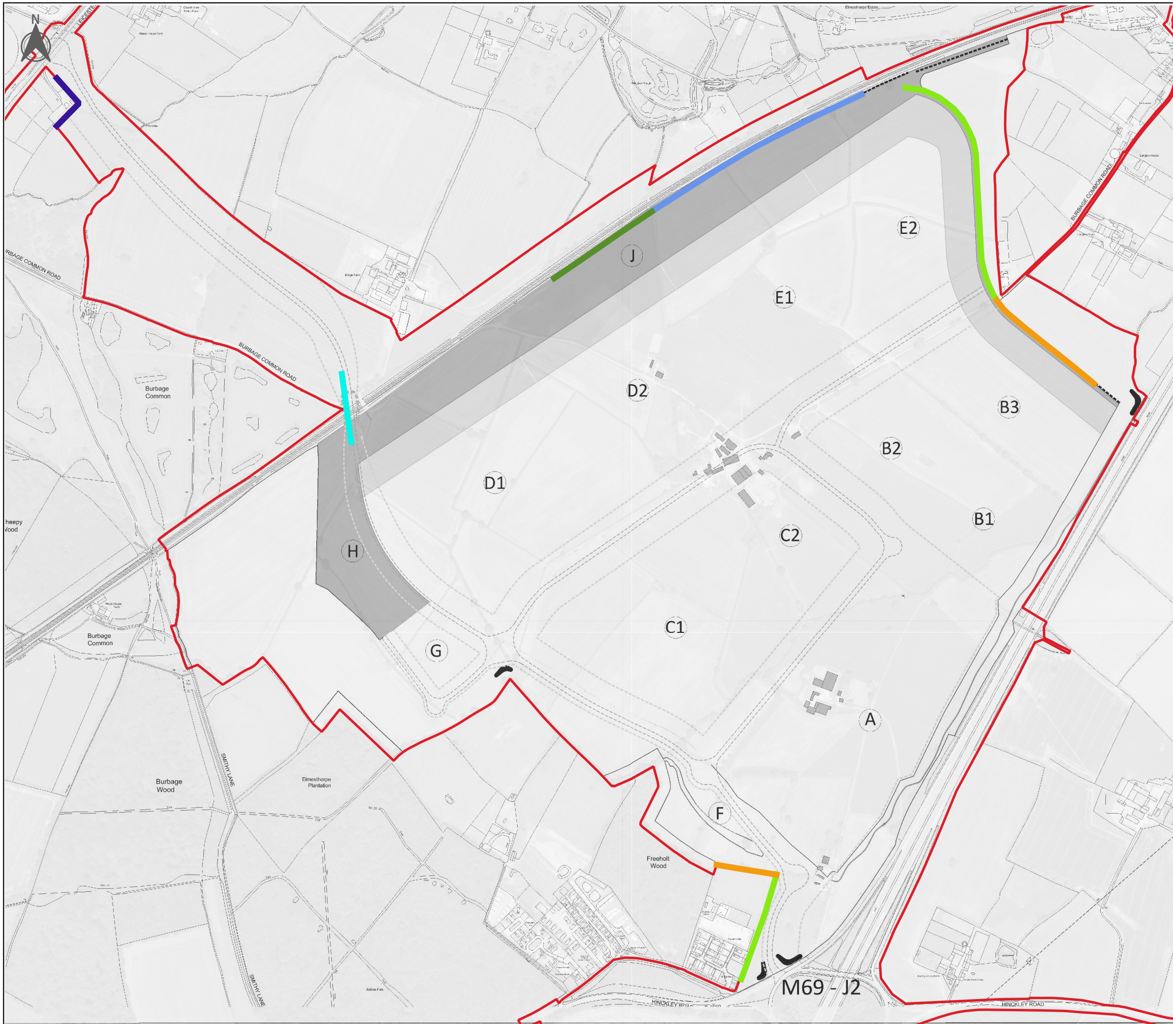
Figure 10.10 - Acoustic Barrier Locations
